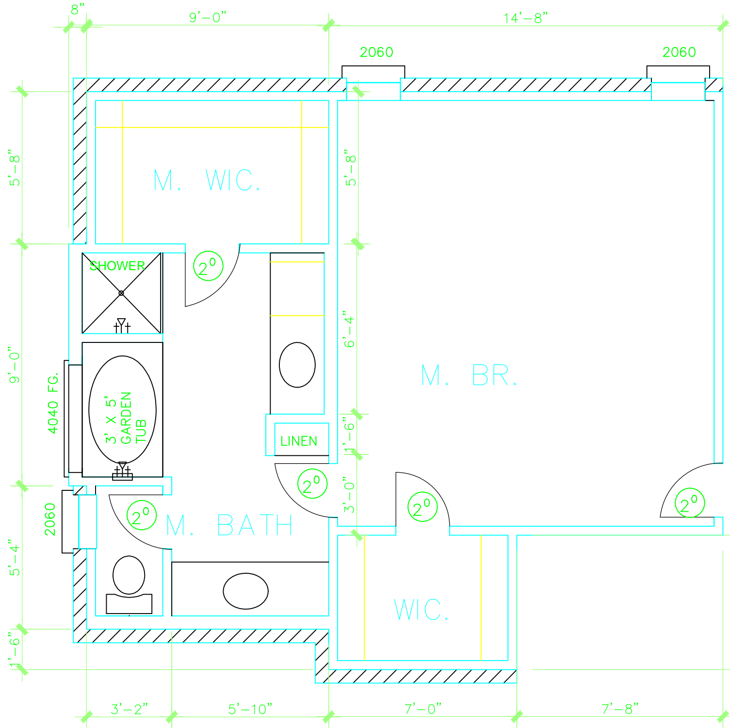
SCALE: 1/4" = 1'-0" FLOOR PLAN
